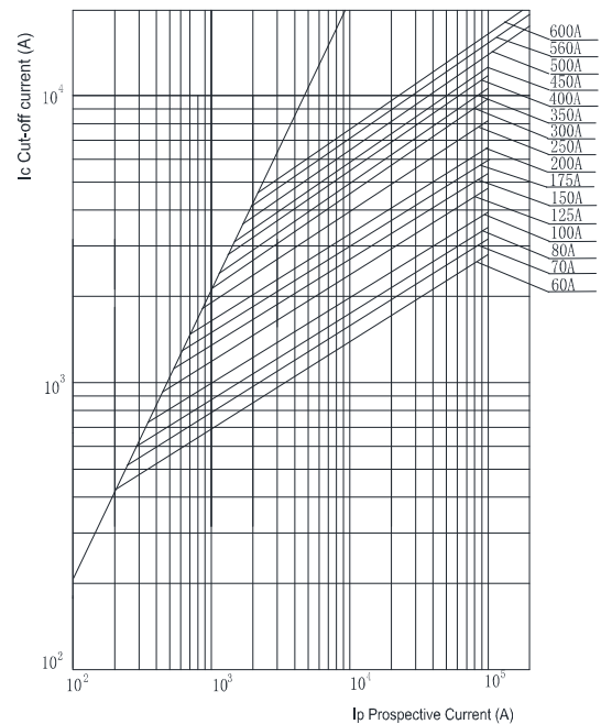
Current Limiting (reference)
