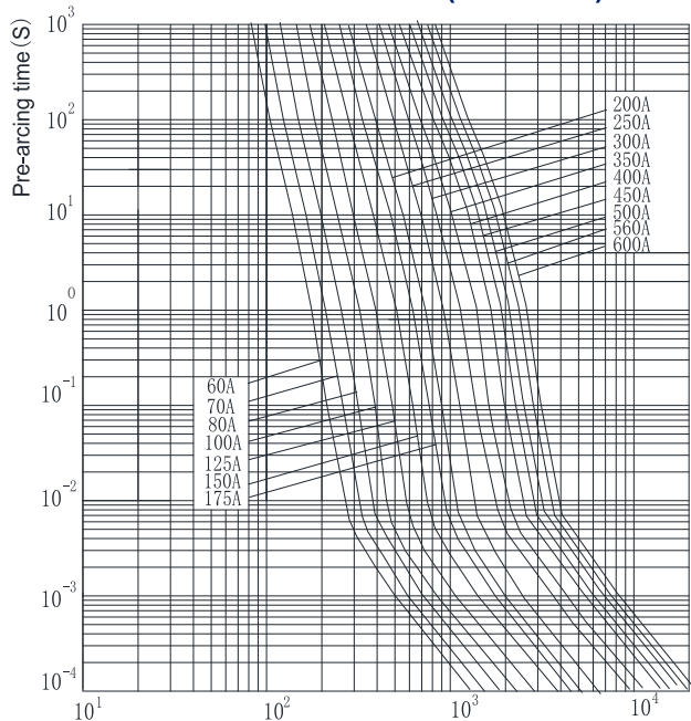
Time Current Curve (reference)
